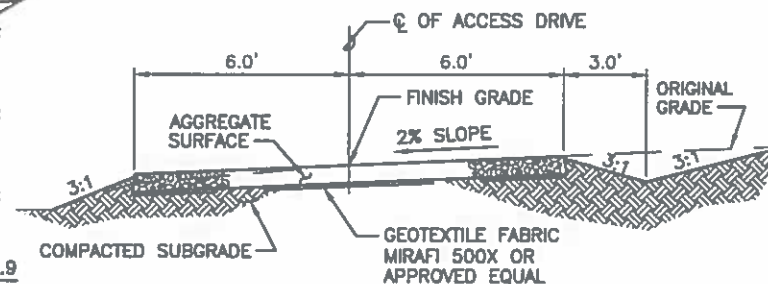
TYPICAL DRIVE SECTION NO SCALE
