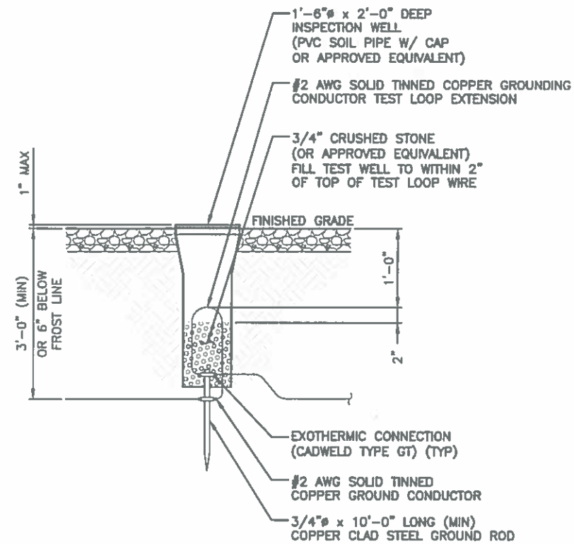
INSPECTION/TEST WELL DETAIL
