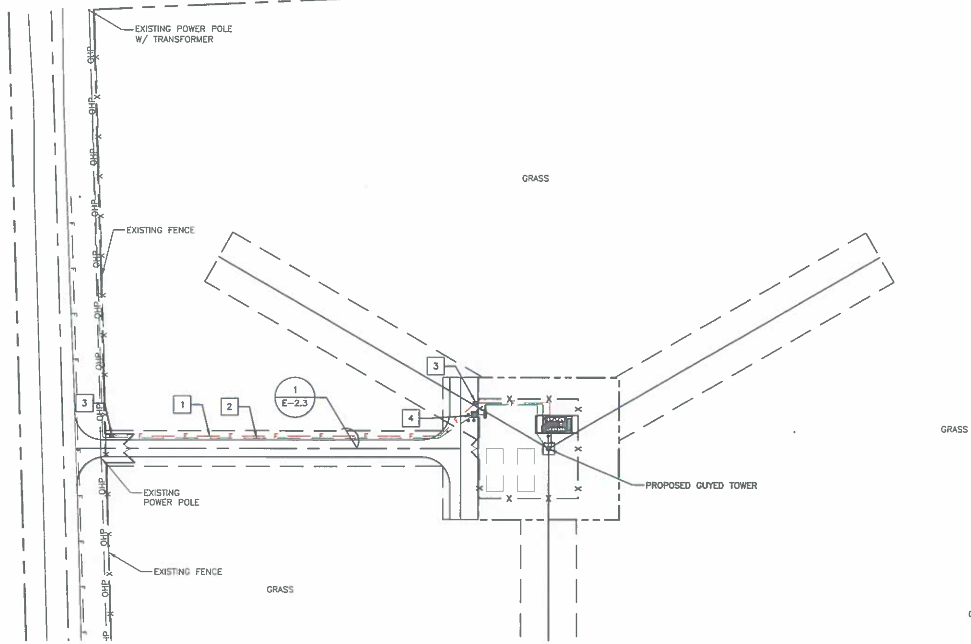
OVERALL UTILITY PLAN
