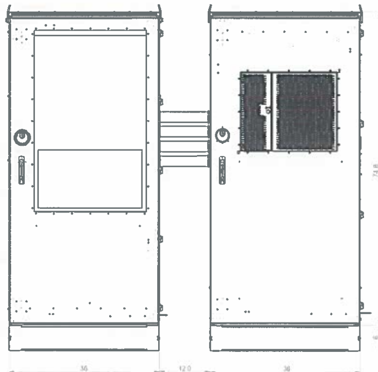
Main equipment cabinet (CMC74-36E)
