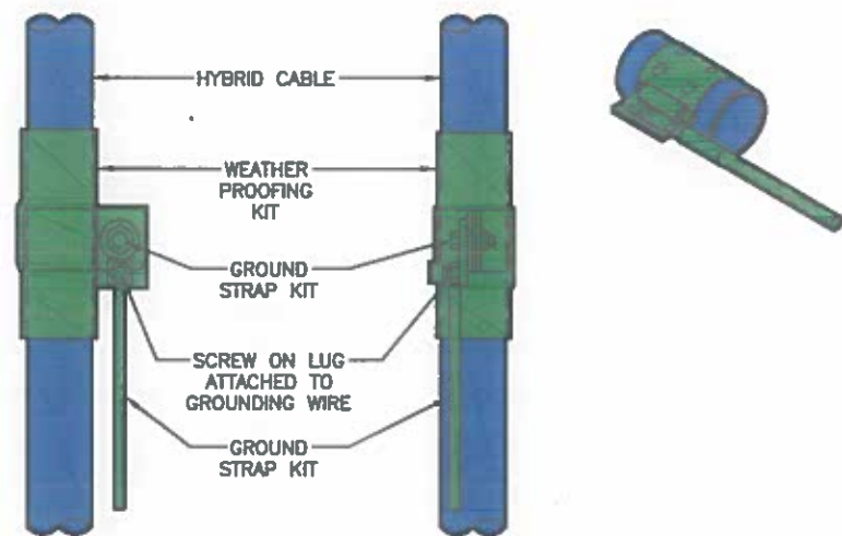
COAX/HYBRID CABLE GROUND KIT DETAIL
