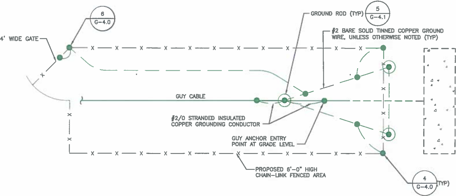
GUY ANCHOR GROUNDING PLAN
