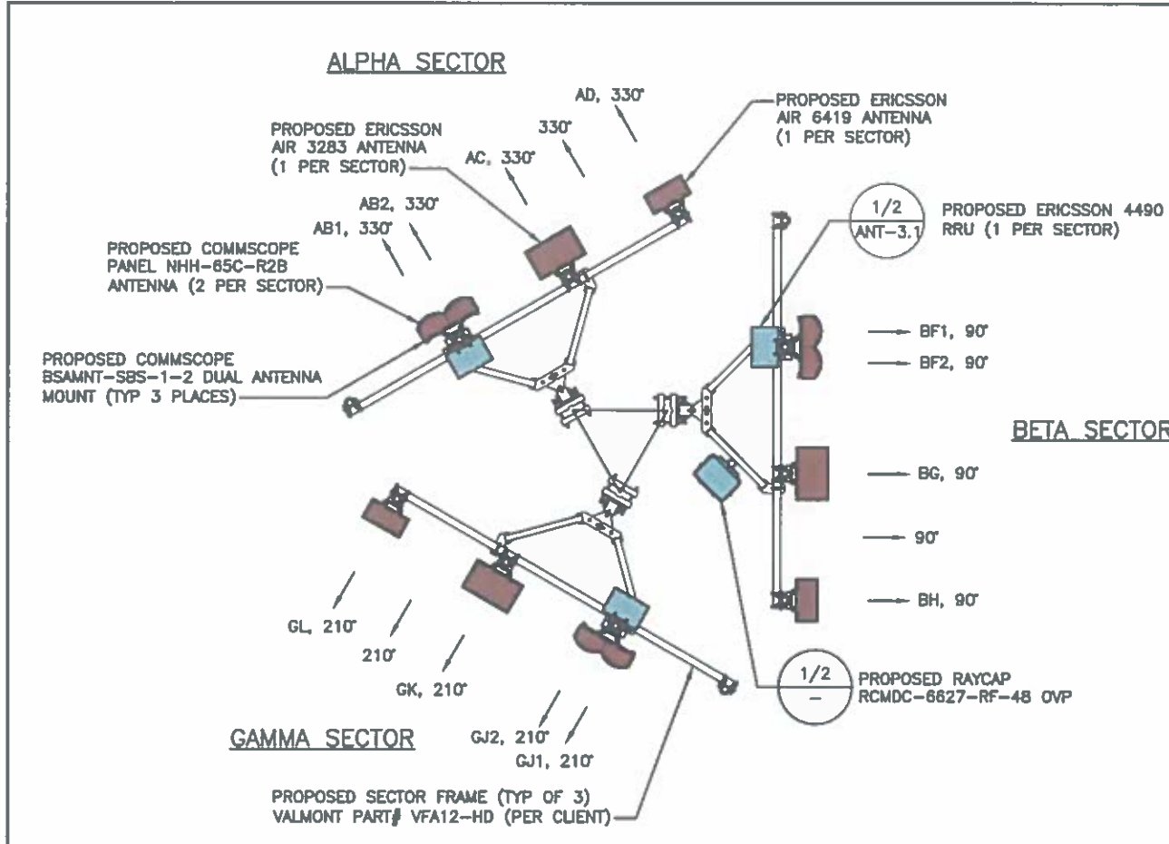
SECTOR EQUIPMENT LAYOUT
