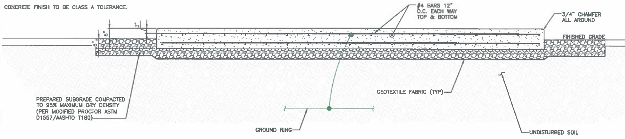
CONCRETE EQUIPMENT PAD (3 CABINETS) - ELEVATION VIEW
