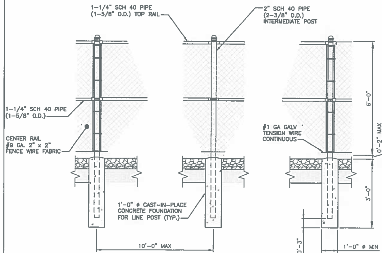
FENCE POST DETAILS
