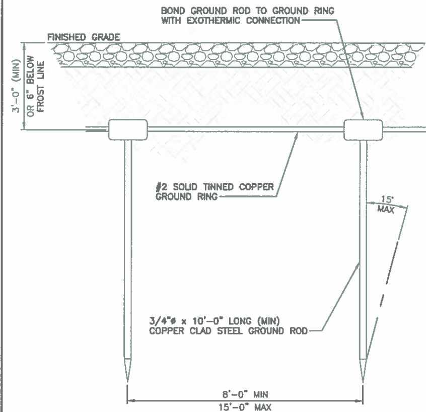
GROUND RING DETAIL
