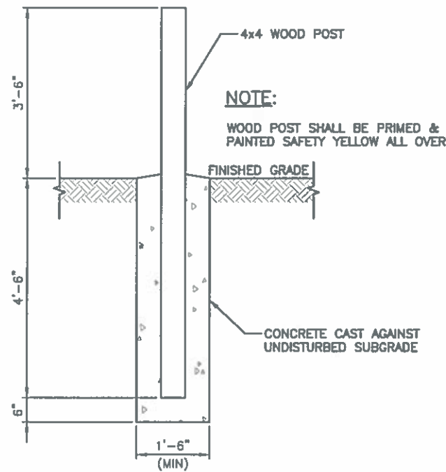
WOOD POST DETAIL
