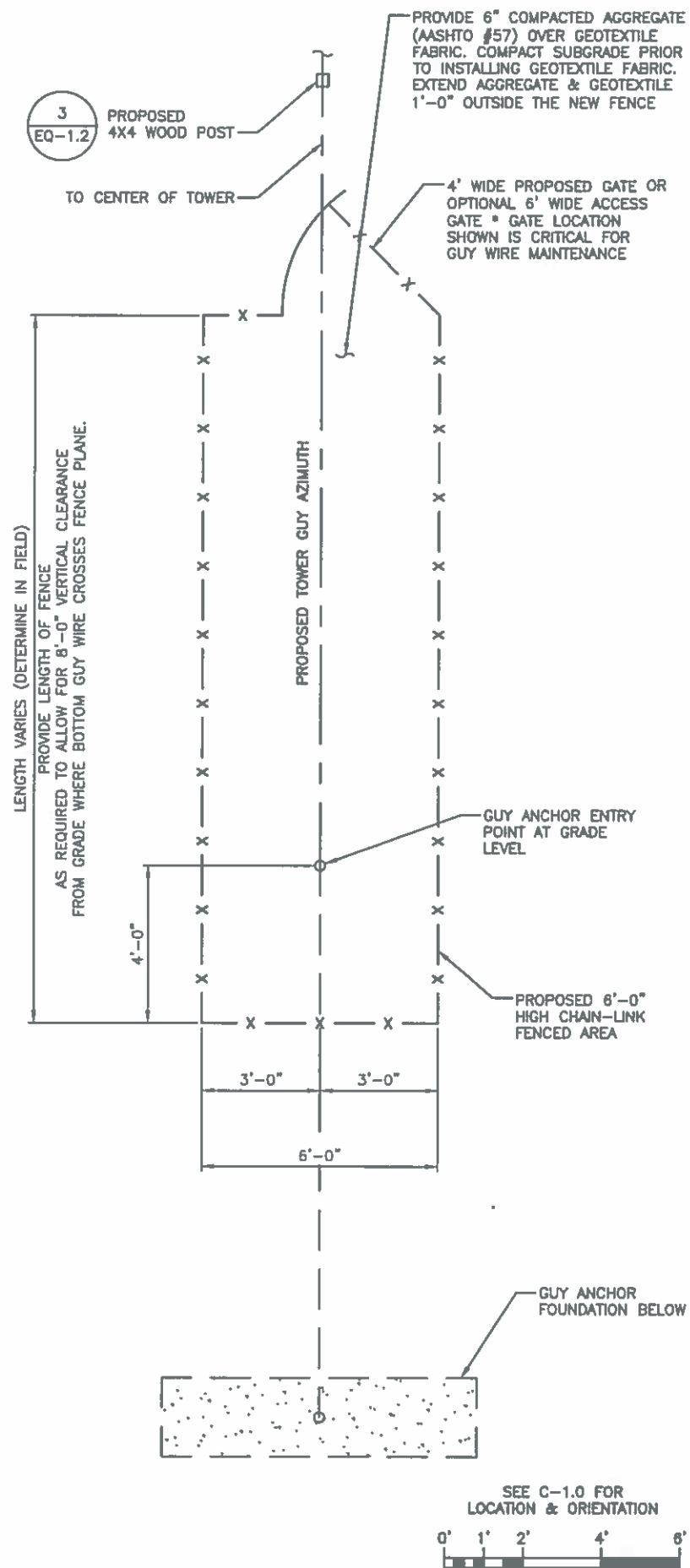
GUY WIRE FENCE PLAN
