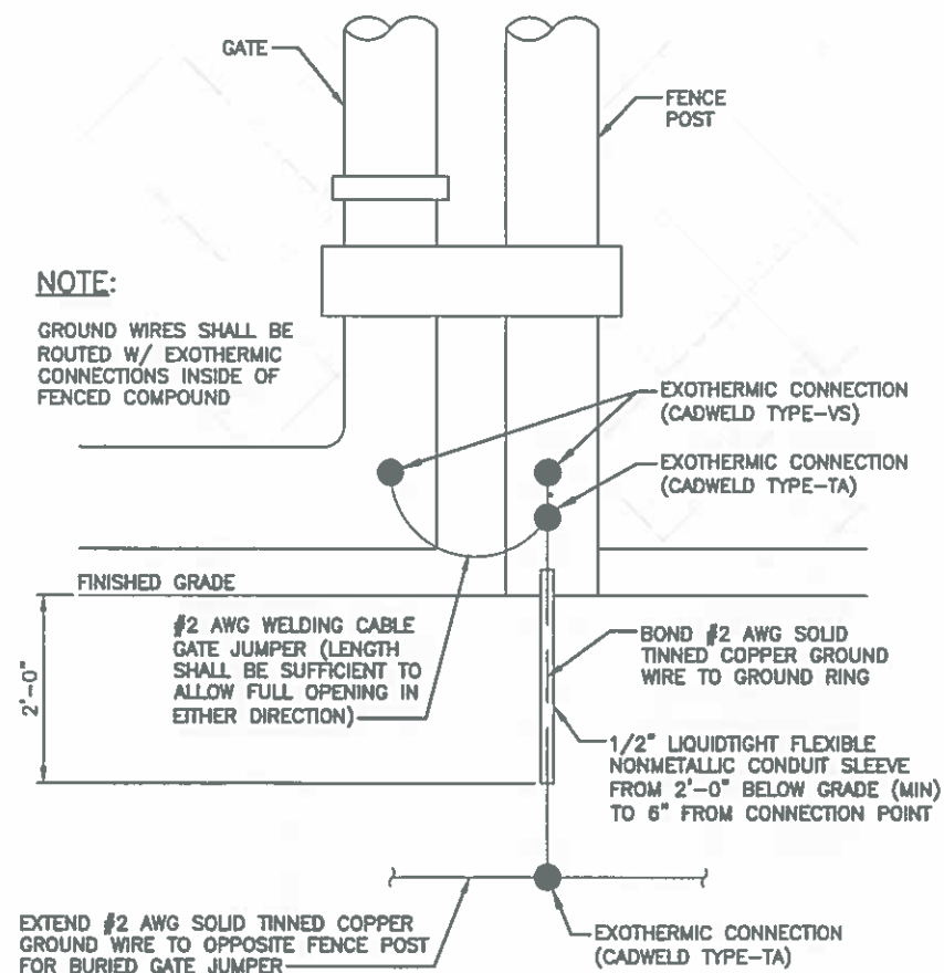
FENCE GATE GROUNDING DETAIL
