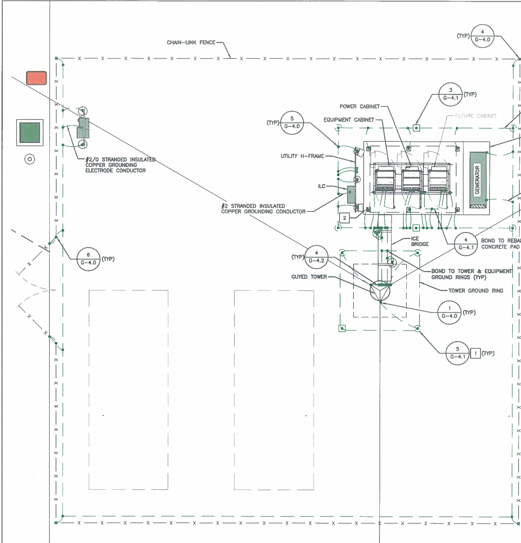
COMPOUND GROUNDING PLAN
