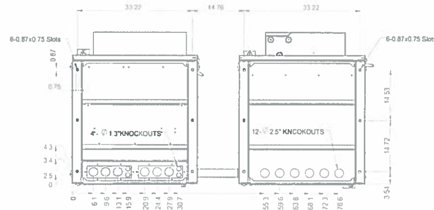
Main equipment cabinet (CMC74-36E)
