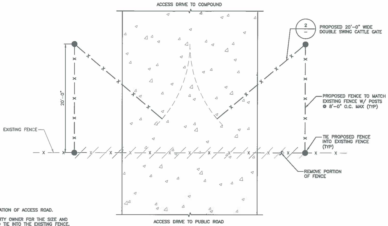
ACCESS GATE PLAN
