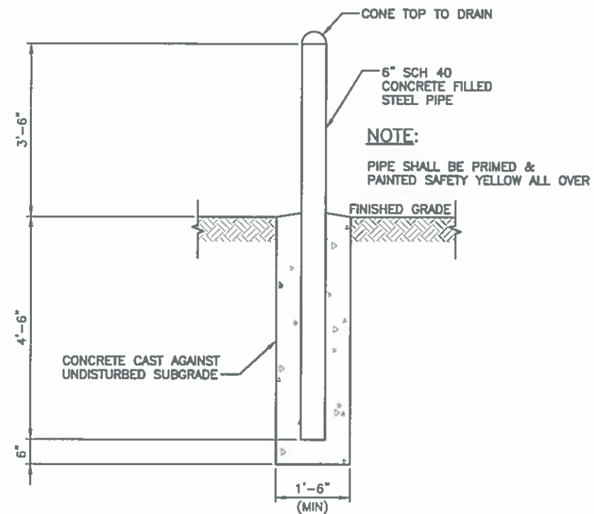
CONCRETE FILLED BOLLARD DETAIL
