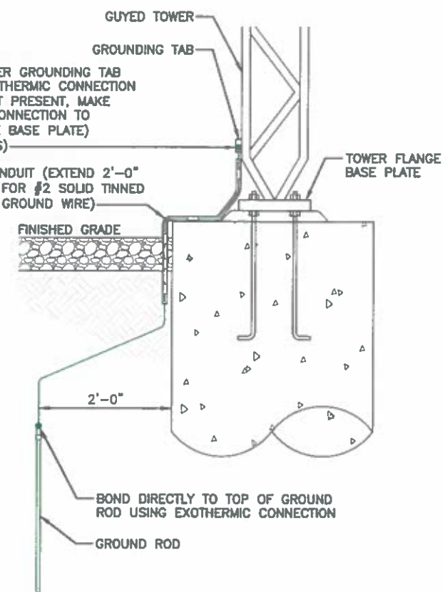
TOWER GROUNDING DETAIL
