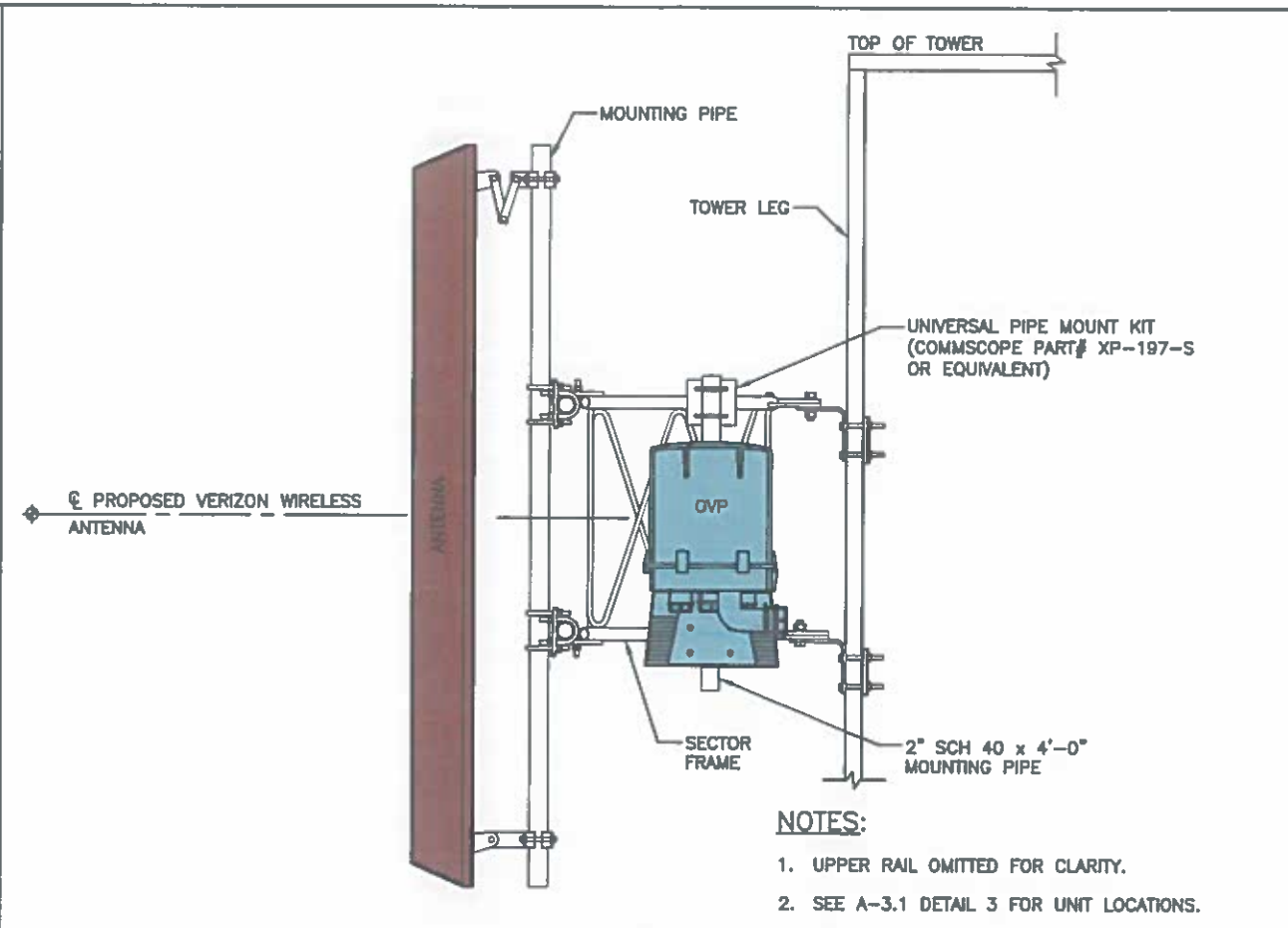
OVP MOUNTING DETAIL
