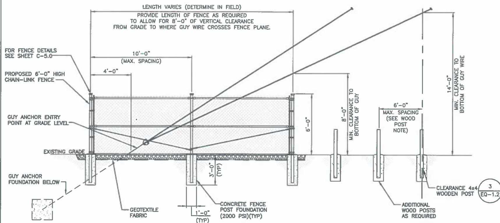
GUY WIRE FENCE SIDE PROFILE
