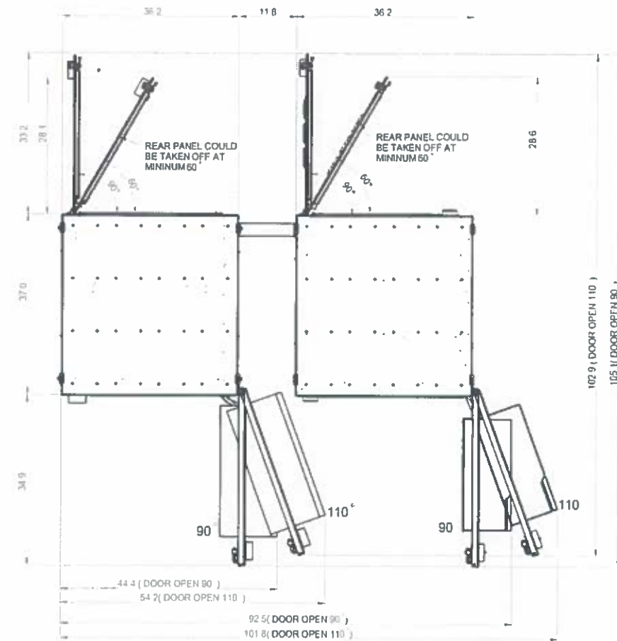
Main equipment cabinet (CMC74-36E)
