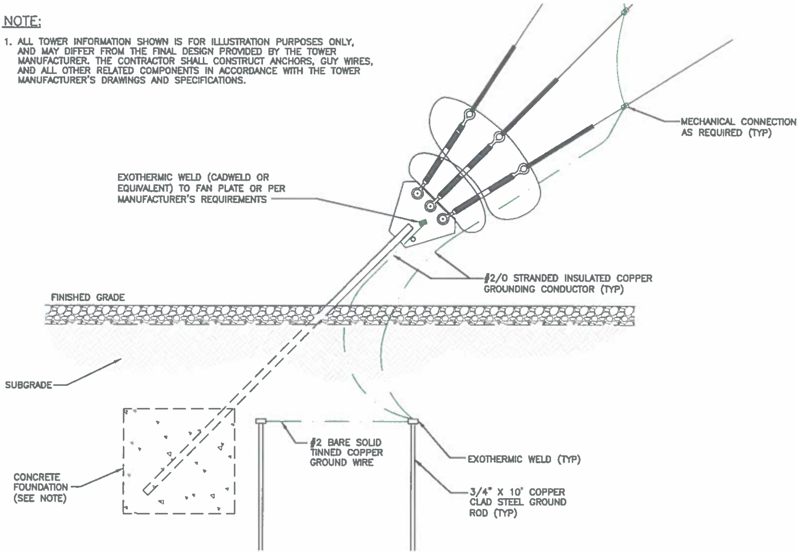
GUY ANCHOR GROUNDING ELEVATION
