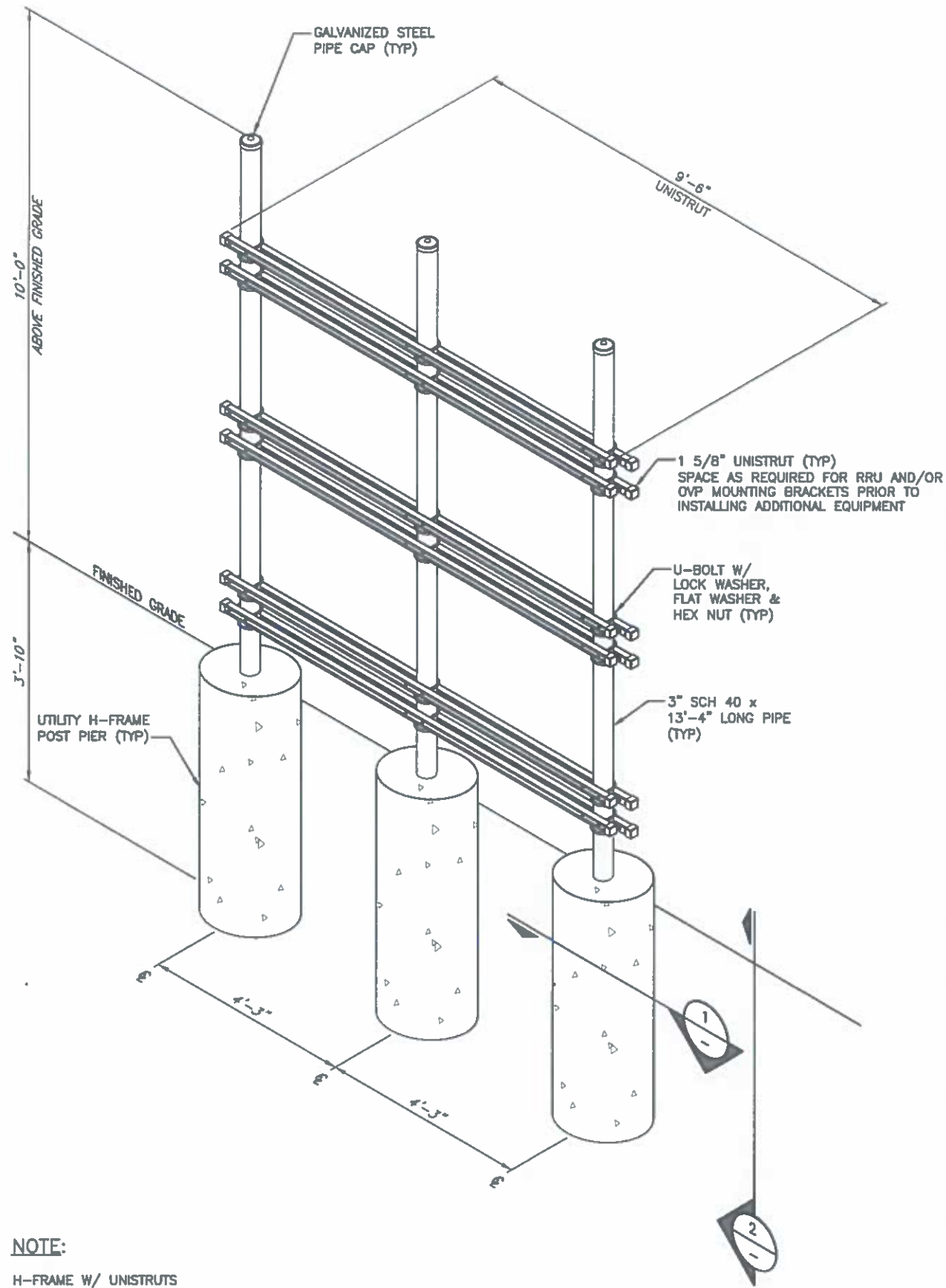
UTILITY H-FRAME DETAIL
