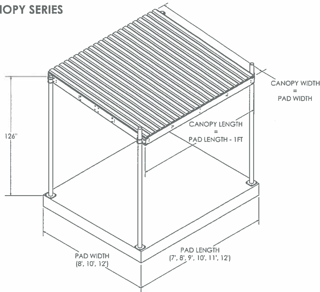
4 POST WEATHER CANOPY
