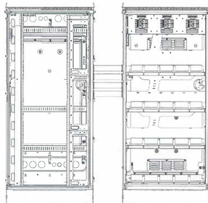
Main equipment cabinet (CMC74-36E)
