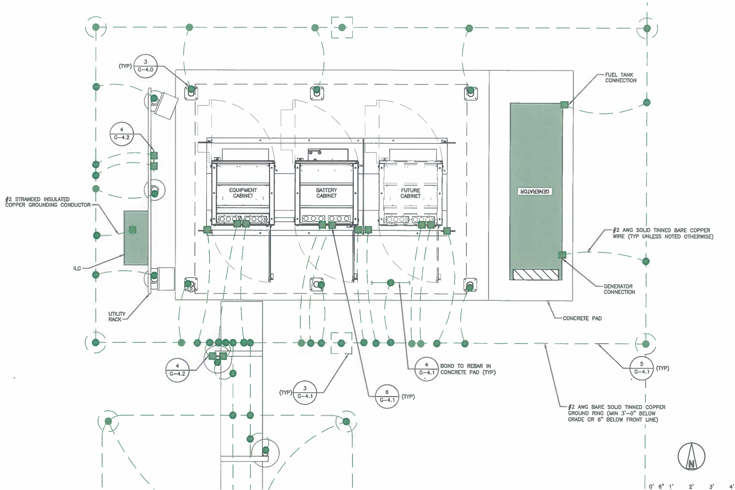
EQUIPMENT GROUNDING LAYOUT
