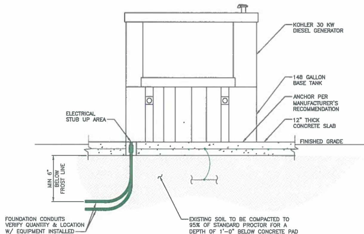
GENERATOR ELEVATION
