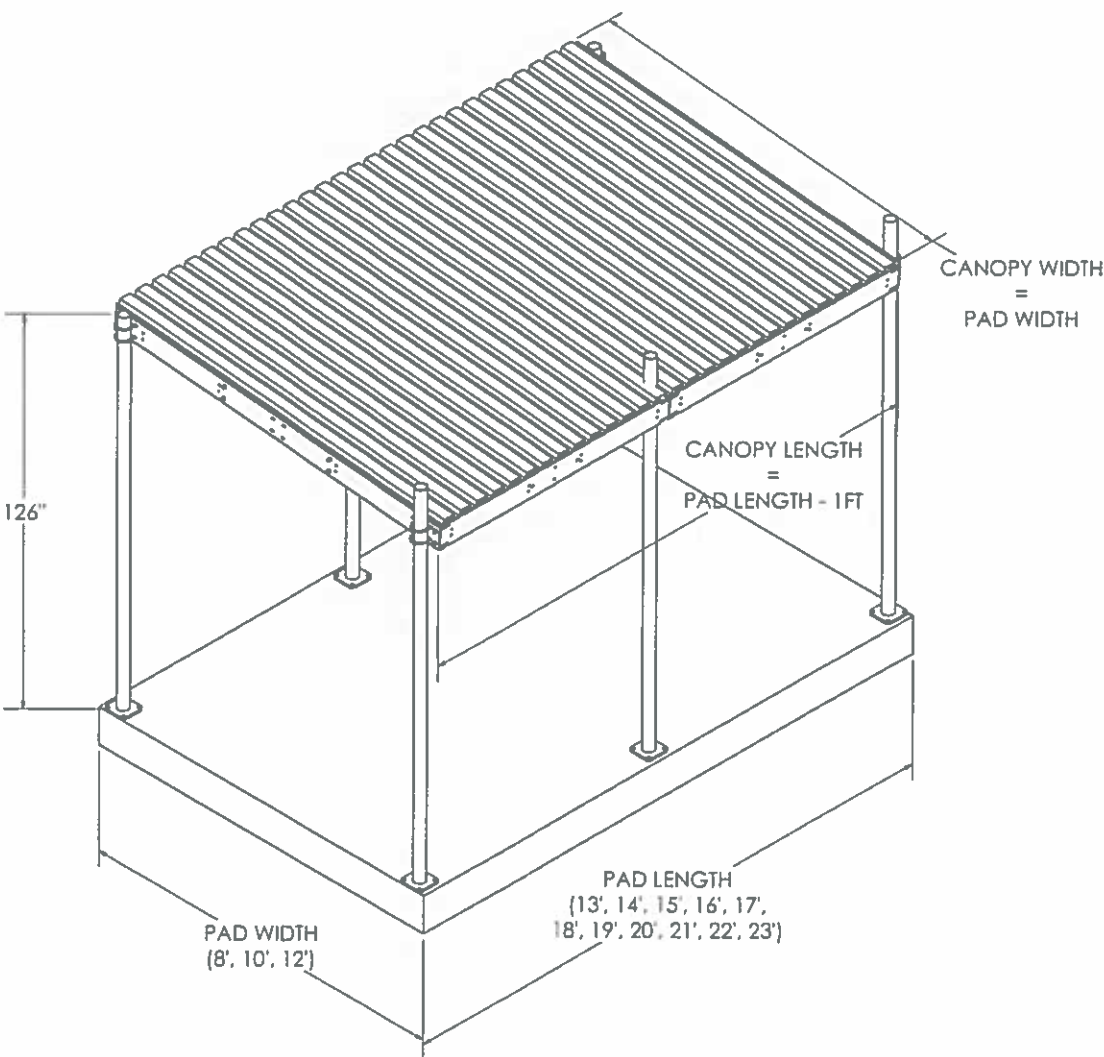
6 POST WEATHER CANOPY
