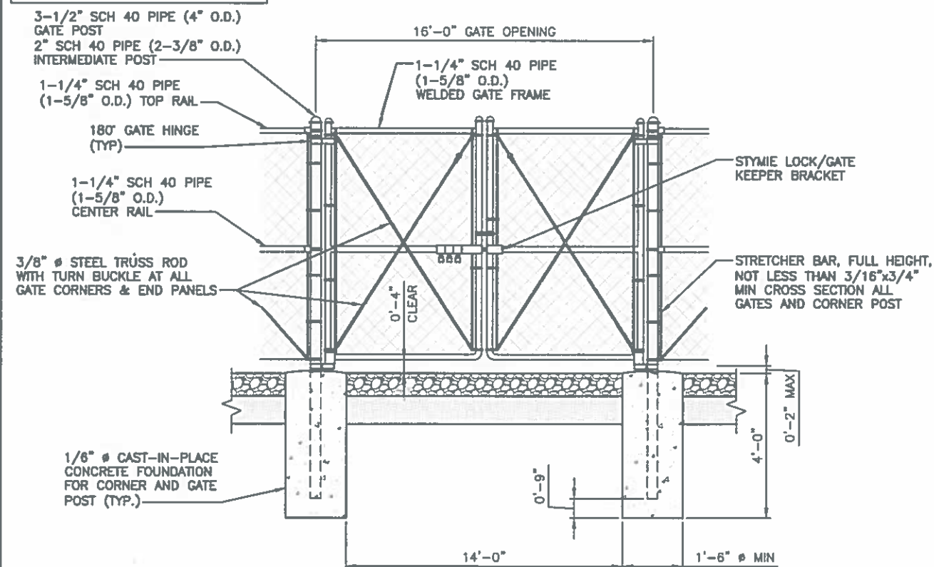
16'-0" DOUBLE SWING GATE DETAIL
