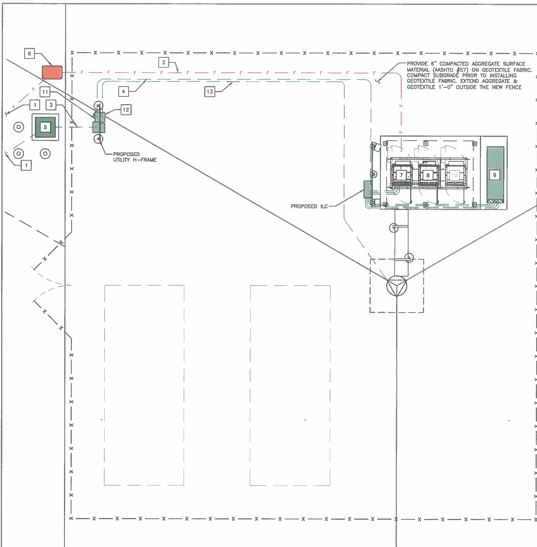
ENLARGED UTILITY PLAN
