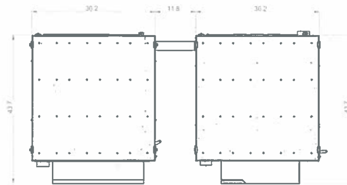
Main equipment cabinet (CMC74-36E)
